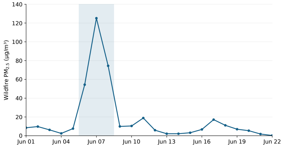
Figure 7: Wildfire smoke exposure in New York, New Jersey, and Pennsylvania, June 2023. The figure shows population-weighted daily wildfire-attributable PM 2.5 concentrations across ZIP3 areas in the three states. Weights are ZIP3 population totals constructed from 2010 Census ZCTA populations. Shading marks June 6–8, the exposure dates used in the back-of-the-envelope calculation. Concentrations measure wildfire-attributable PM 2.5 rather than total PM 2.5 .
