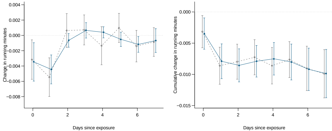
Figure J.21: PM-specific AQI dynamics: running minutes. OLS responses to a one-day increase of ten points in PM-specific AQI. Gray dashed lines with open circles show unrestricted seven-day estimates; blue solid lines with squares show seven-day spline estimates. The left panel shows the response at each lag. The right panel shows the cumulative response through each lag. Models include temperature and precipitation categories, daylight duration, participant, ZIP3-by-month-by-year, and calendar-date fixed effects. Bars show 95% confidence intervals based on standard errors clustered by reporting area and calendar date.
