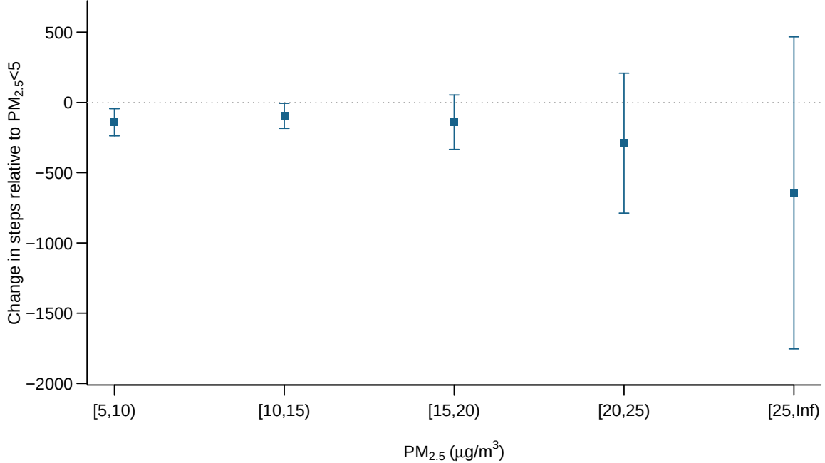
Figure 4: Daily steps across separate pollution intervals. Each estimate compares the indicated PM 2.5 interval with [0, 5) \mu\text{g}/\text{m}^3 in a separate restricted sample, instrumenting the comparison indicator with the cross-fitted selected-direction instrument. Bars show 95% confidence intervals based on standard errors clustered by ZIP3 and calendar date.
