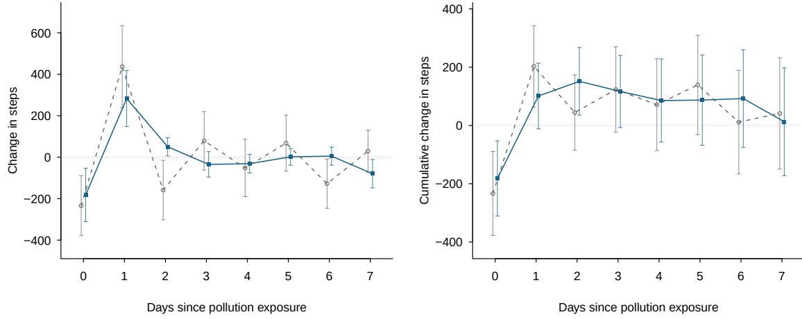
Figure 2: Dynamic step responses: continuous \text{PM}_{2.5} . Exposure is a one-day increase of 10 \mu\text{g}/\text{m}^3 . Gray dashed lines with open circles show unrestricted lag estimates; blue solid lines with squares show spline estimates. The left panel shows the response at each lag. The right panel shows the cumulative response through each lag. Bars show 95% confidence intervals based on standard errors clustered by ZIP3 and calendar date.
