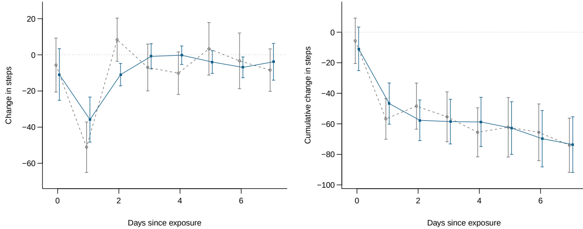
Figure 5: Dynamic step responses to wildfire smoke. The exposure is a one-day increase of 10 \mu g/m^3 in wildfire PM_{2.5} . Gray dashed lines with open circles show unrestricted seven-day estimates; blue solid lines with squares show seven-day spline estimates. The left panel shows the response at each lag. The right panel shows the cumulative response through each lag. Both models are estimated by OLS with temperature and precipitation categories, daylight duration, participant, ZIP3-by-month-by-year, and calendar-date fixed effects. Bars show 95% confidence intervals based on standard errors clustered by ZIP3 and calendar date.
